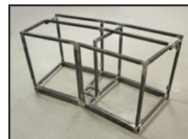
Welded and ground Frame ready for powder coat
